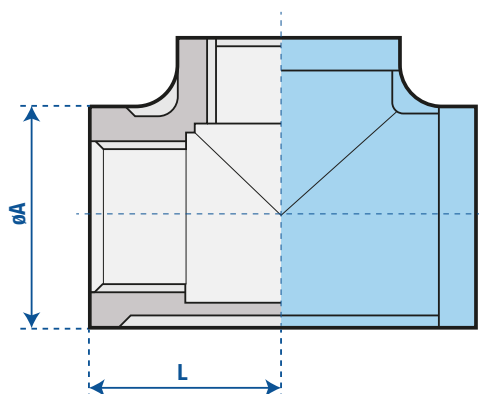
Equal Female Tee
