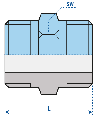
Equal Hexagon Nipple
