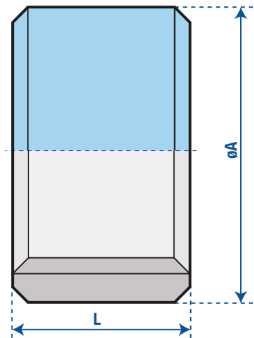
Half Socket (Coupling) O.D. Machined
