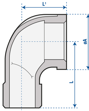
Equal M/F 90 Street Elbow
